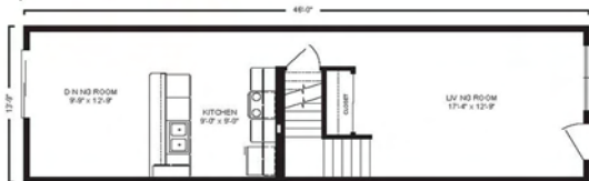
FIRST FLOOR
